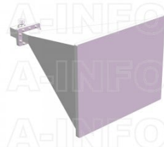
LB-284-20-C-7/16FSP Standard Gain Horn Antenna 2.6-3.95GHz 20dB Gain 7/16(DIN) Female
