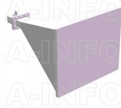
LB-284-20-C-NFSPS Standard Gain Horn Antenna 2.6-3.95GHz 20dB Gain N Type Female
